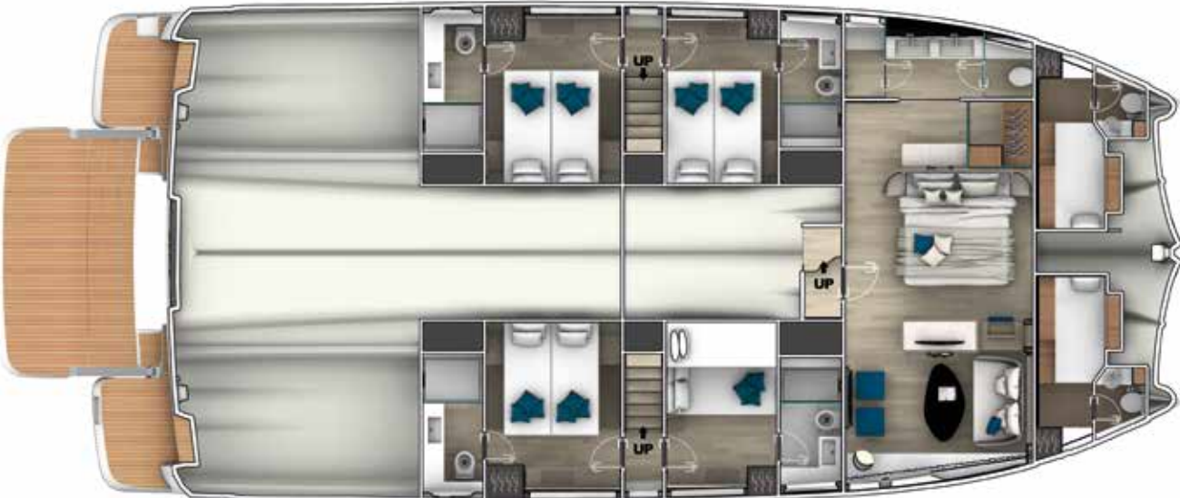
Galley up layout 5 staterooms, 5 bathrooms
